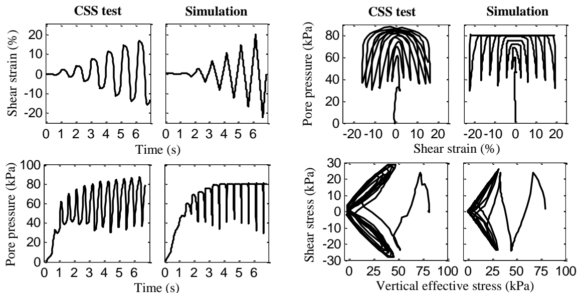
Figure 3. 5. Comparison of the simulated and measured response during a Cyclic Simple Shear (CSS) test performed on ( D_r=63\% , \sigma'_{v0}=80 kPa, and CSR=0.3 ).
