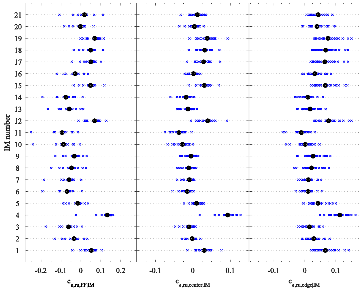
Figure 6. 16.The slope ( c ) values corresponding to the linear regression of residuals in r_{u,peak} for a given candidate IM as a function of source M_w . The blue crosses indicate individual c values and the black circles show the average c among the twenty one simulations.
